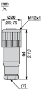
(1) Cable gland : no. 7 plastic (Pg 7)
